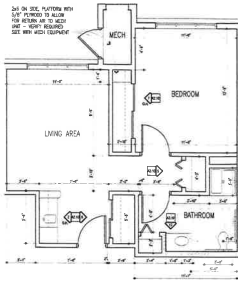
5 Detail - One Bedroom A1.04 SCALE: 1/8" = 1'-0" REF:
