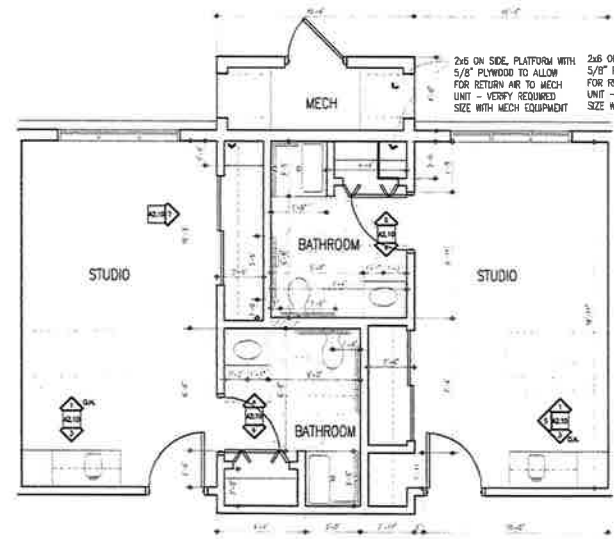
3 Detail - Studio A1.04 SCALE: 1/8" = 1'-0" REF:
