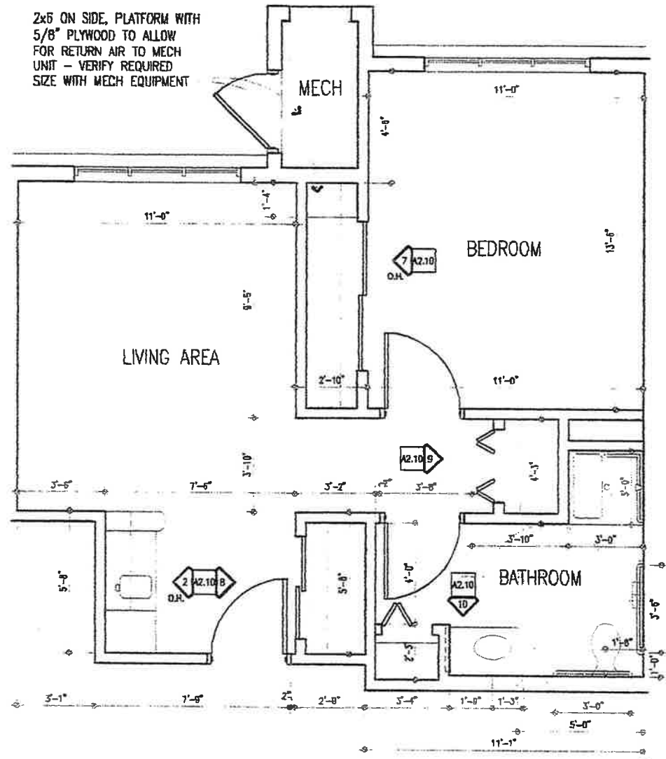
5 Detail - One Bedroom A1.04 SCALE: 1/4" = 1'-0" REF:
