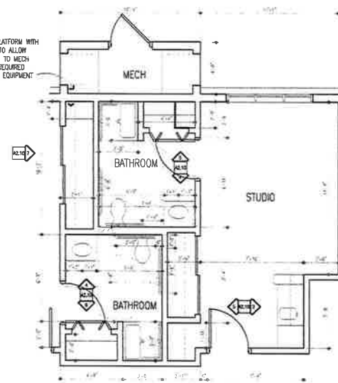
2 Detail - Studio A1.04 SCALE: 1/8" = 1'-0" REF:
