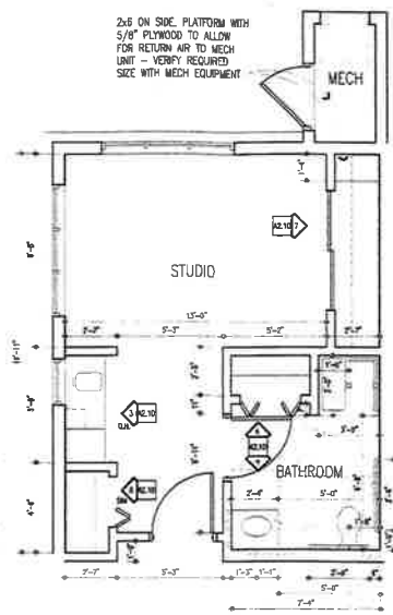
4 Detail - Studio A1.04 SCALE: 1/8" = 1'-0" REF:
