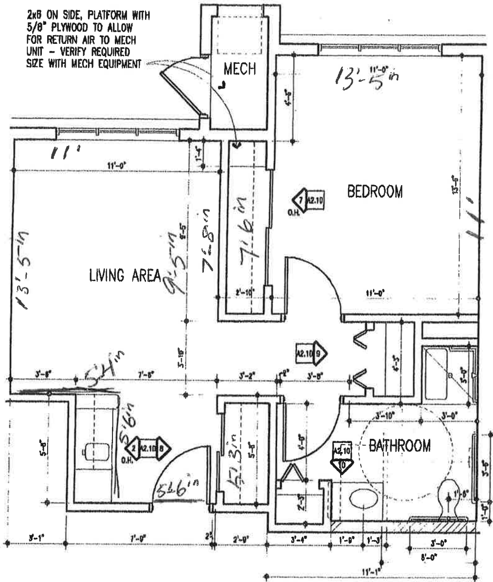
5 Detail - One Bedroom A1.04 SCALE: 1/4" = 1'-0" REF:
